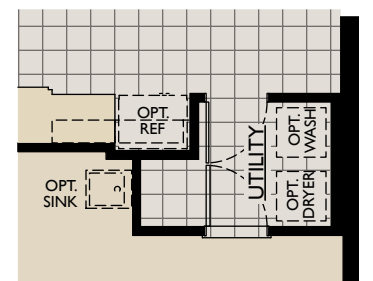
OPT. LAUNDRY NICHE
